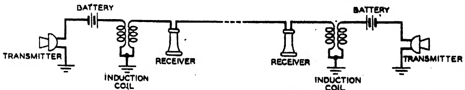
FIG. 6. EARLY TELEPHONE CIRCUIT (WITH MICROPHONE AND BATTERY) A SINGLE WIRE WAS USED; THE RETURN WAS THROUGH THE GROUND. THE INDUCTION COIL KEPT THE BATTERY CURRENT OFF THE LINE, THUS PERMITTING LARGER CHANGES IN THE RESISTANCE OF THE BATTERY CIRCUIT AND STRONGER VOICE CURRENTS. WITH THIS TYPE OF CIRCUIT AND A RETURN WIRE, TELEPHONE CONVERSATION WAS CARRIED ON BETWEEN NEW YORK AND CHICAGO IN 1892.
